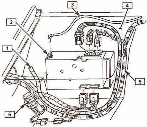
15.19 Radio receiver mounting details - 1990 and later models
