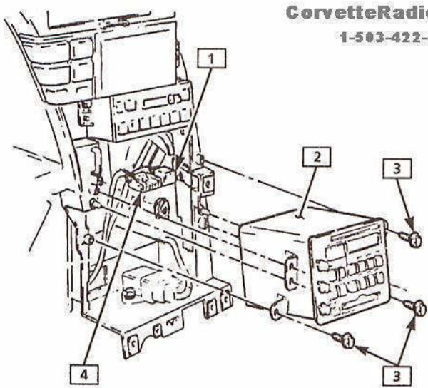
15.17 Radio control mounting details - 1990 and later models
